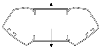
A Direct/Indirect Micro Prismatic Diffuser
